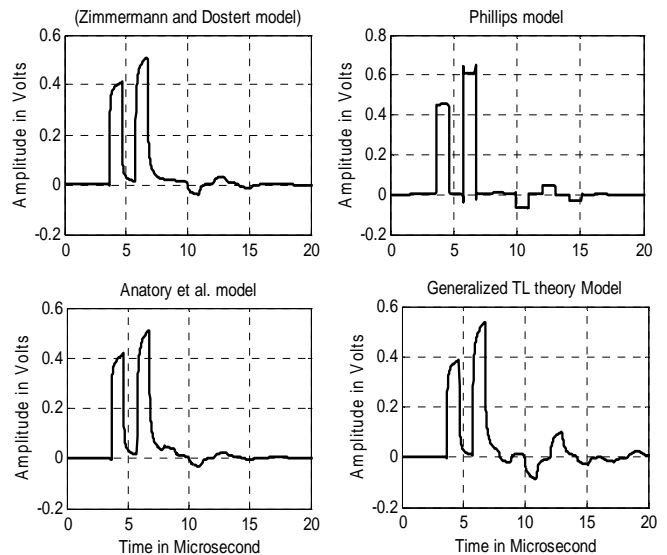
Fig. 6 Comparisons for power line channel models with Zimmermann and Dostert [5] improved for a power line network with two distributed branches with terminal loads terminated in 10M-ohms [11]
