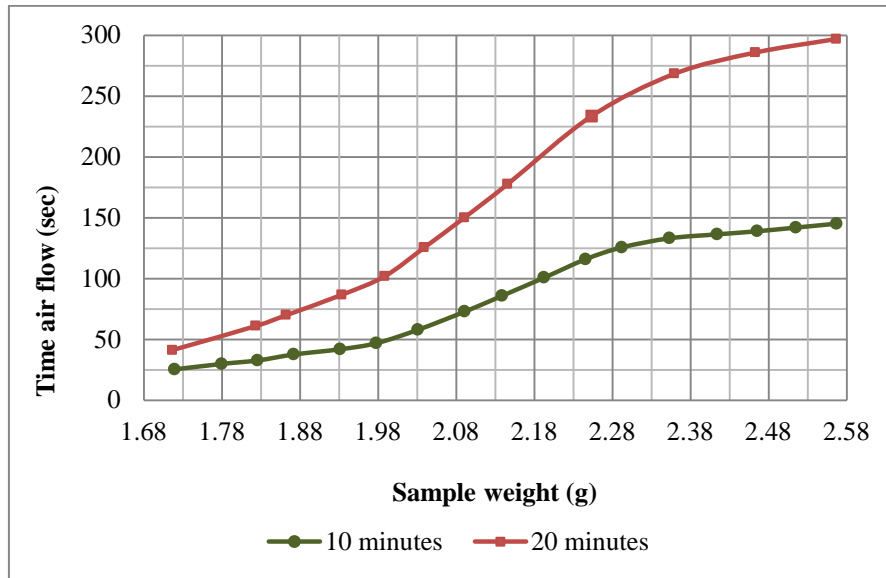
Figure 3: Graphs of time air flows versus weights of pozzolan at different milling duration
