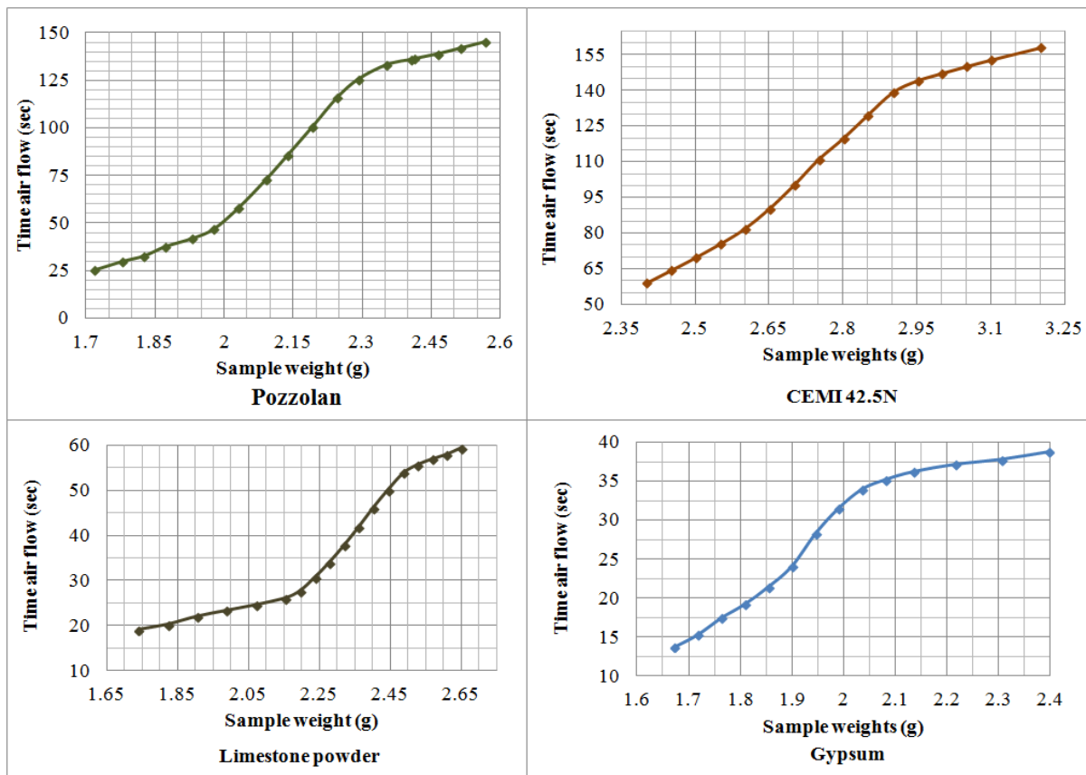
Figure 2: Graphs of time air flows versus weights of samples for various powder materials
