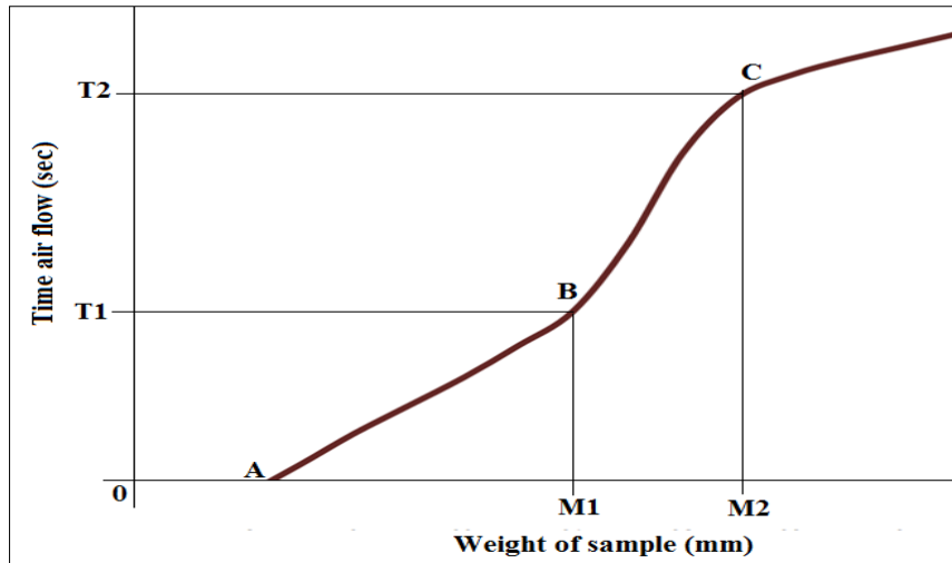
Figure 1: Graph representing time air flow versus weight of sample in a tin
