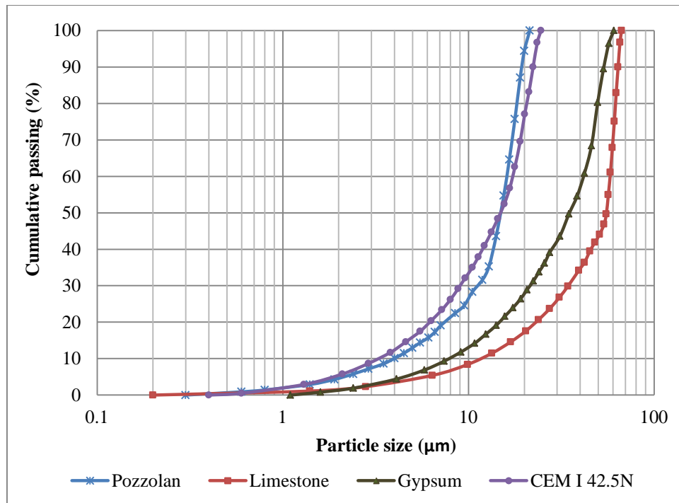
Figure 4: Synthetic particle size distribution of powder materials
