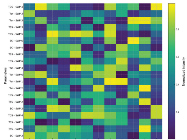
Figure 10. Heatmap for physicochemical (EC, TDS, Tur, and TSS) parameters
