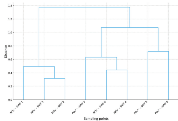
Figure 5. Dendrogram showing hierarchical clustering of phosphate ( \text{PO}_4^{3-} ) and nitrate ( \text{NO}_3^- ) concentrations across six surface water points (SWP 1–SWP 6) in the Tunduma watershed
