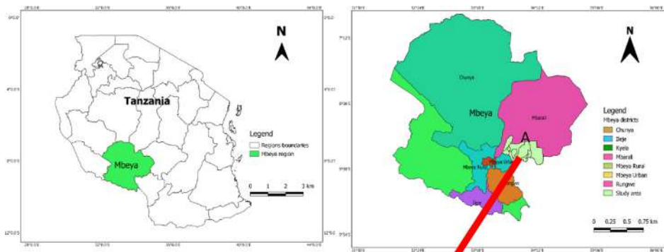
Fig. 1. Distribution of soil sampling sites in different irrigation schemes of the Usangu basin-Mbeya Tanzania.
