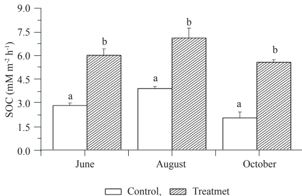
Fig. 4. Sediment oxygen consumption (SOC) rates recorded in the treatment and the control ponds during the experimental period. Data expressed as means \pm SE, n=3. Means that are not sharing a common alphabet are significantly different ( p < 0.05 )
