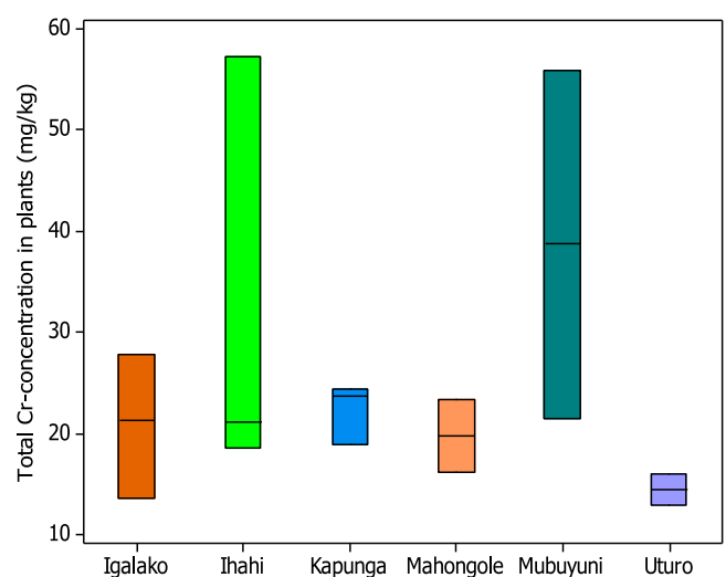
Fig. 5. The Cr accumulation (mg/kg) in paddy rice plants in six irrigation schemes in the Usangu agro-ecosystem (this includes Cr in roots, straws, and grains).
