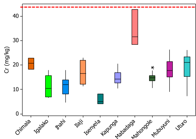
Fig. 4. The Cr distribution in agricultural soils among various irrigation schemes of Usangu agro-ecosystem. Values above the red dotted lines represent exceedance of FAO maximum permissible limits (1 mg/kg). (For interpretation of the references to colour in this figure legend, the reader is referred to the Web version of this article.)
