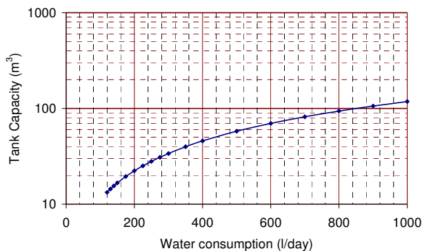
Figure 1. Water consumption against tank capacity.
