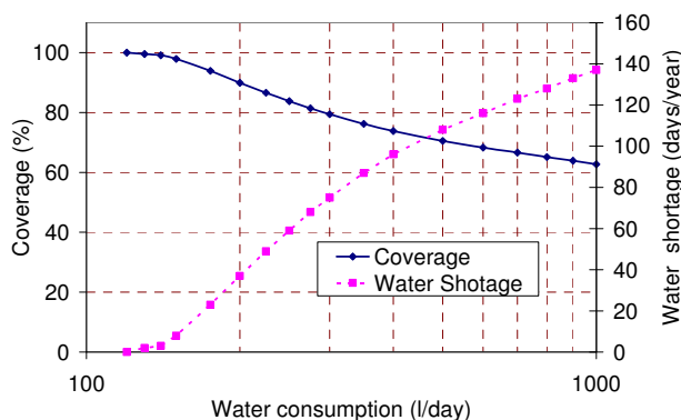
Figure 1. Coverage and number of water shortage days per year against the water consumption per days.
