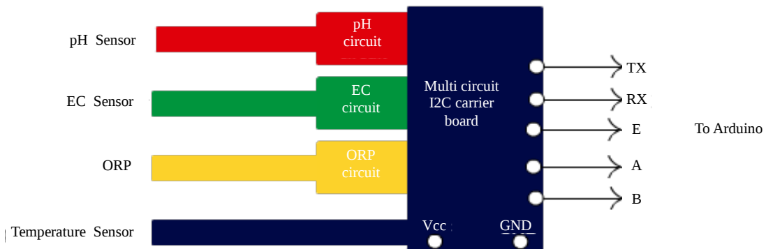
Figure 4. Sensor unit.
