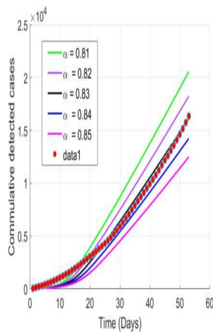
Fig. 7. The model (2) fitted to Ebola cases reported in Guinea from 22 March to 16 August 2014 at \alpha = 0.83 .
