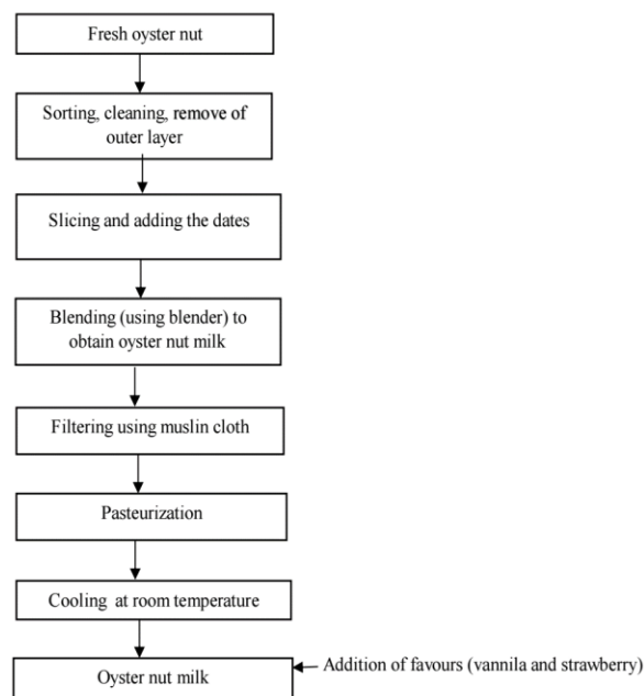
Flow Diagram of Oyster Nut Milk Processing
