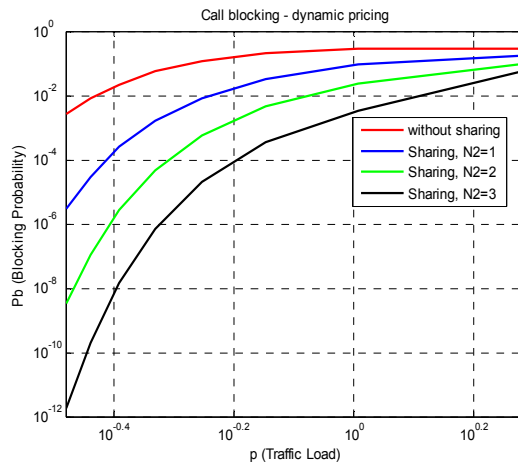
Figure 3: Call blocking for a dynamic priced network with and without spectrum sharing
