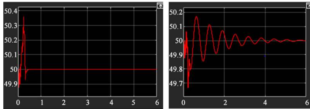
Figure 3. Frequency control at grid connected mode and islanding mode respectively.
