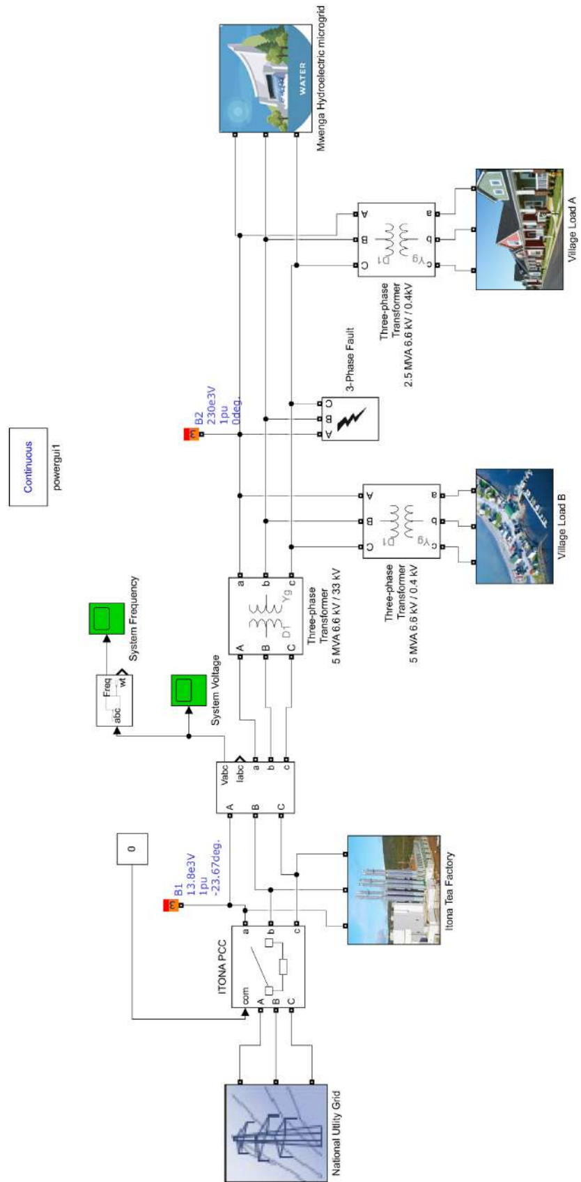
Figure 2. Mwenga grid connected hydroelectric microgrid model.
