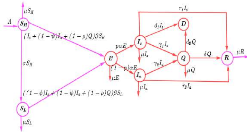
Figure 1: Model flow chat illustrating the dynamics of COVID-19
